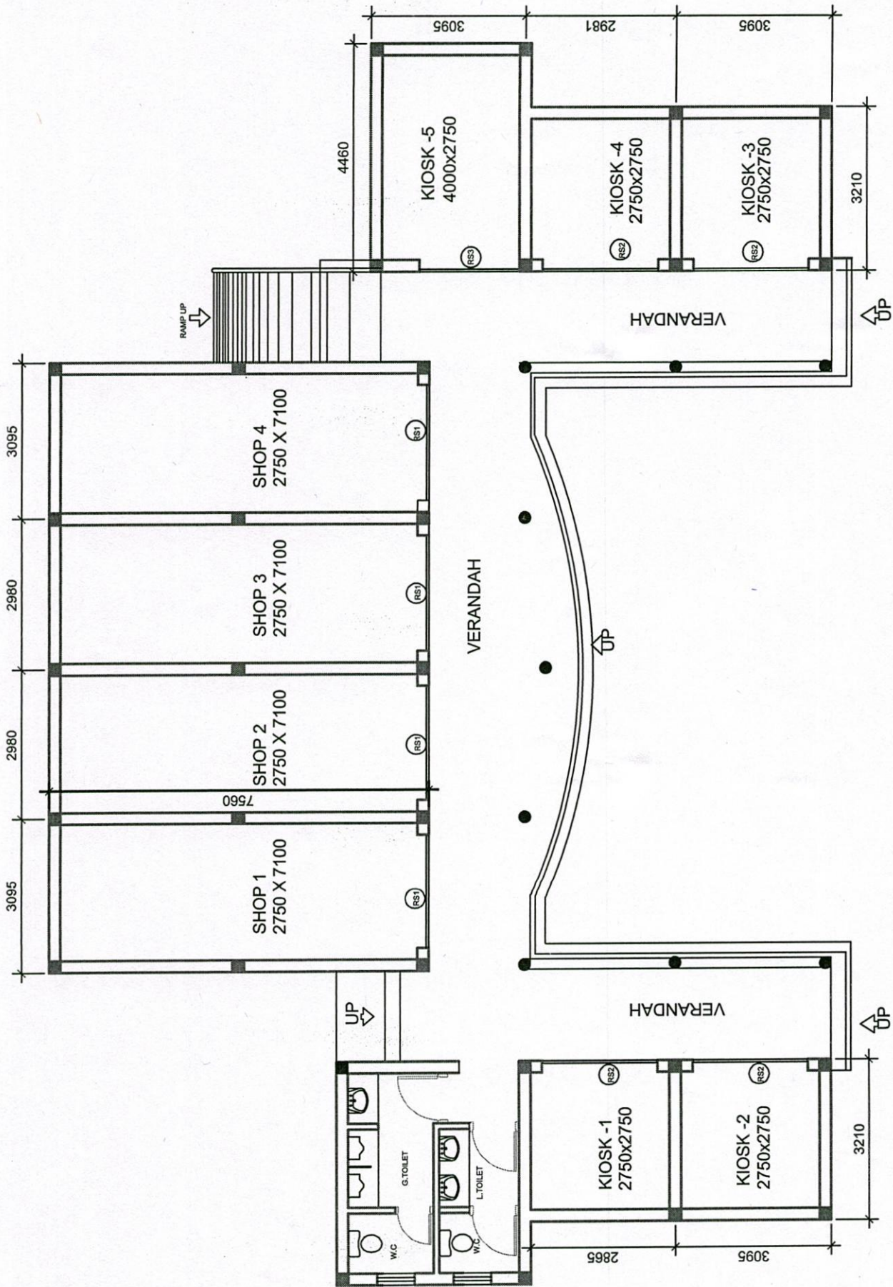
GROUND FLOOR PLAN PLAN OF SHOPS/KIOSKS AT SECTOR-89
